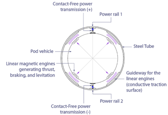
Cross section of the infrastructure
