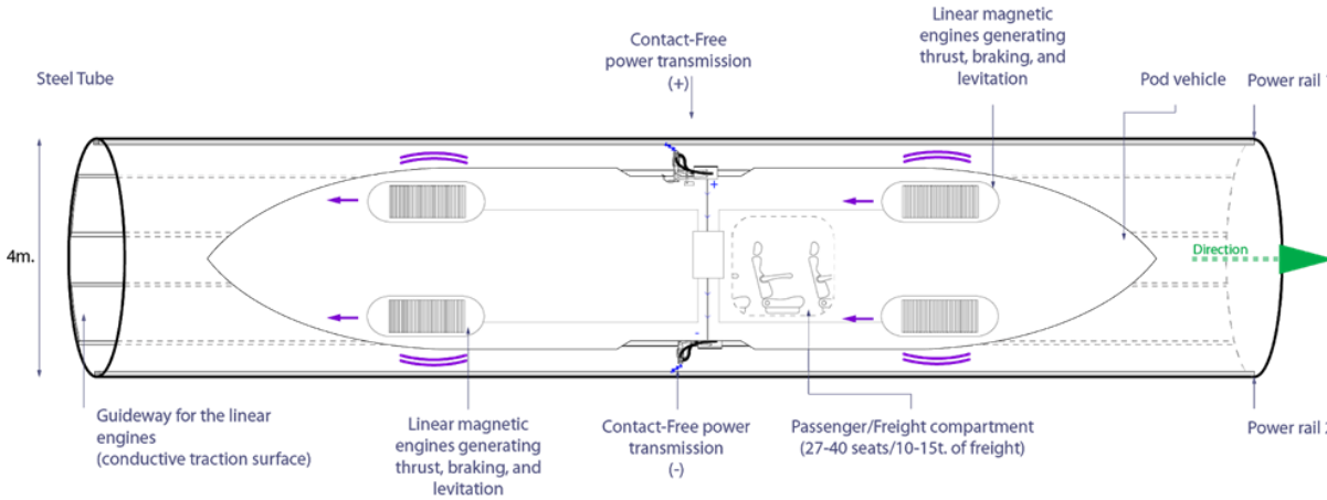
Side view of the pod vehicle
